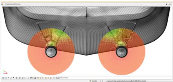
Fig.4: CFD for wake and propulsion improvement source: www.friendship-system.de
