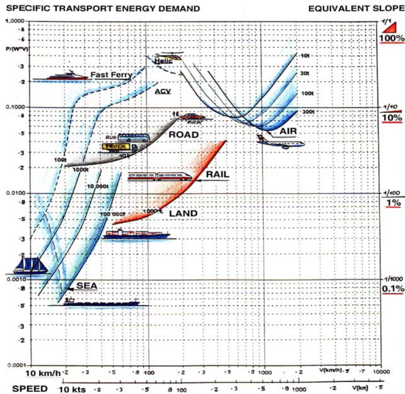
Fig.1: Transport efficiency vs speed for various vessels (modified Karman-Gabrielli diagram)
