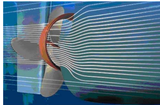
Fig.5: Mewis duct
