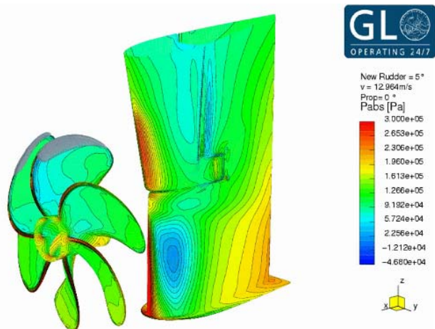
Fig.3: CFD for fuel efficient rudders
