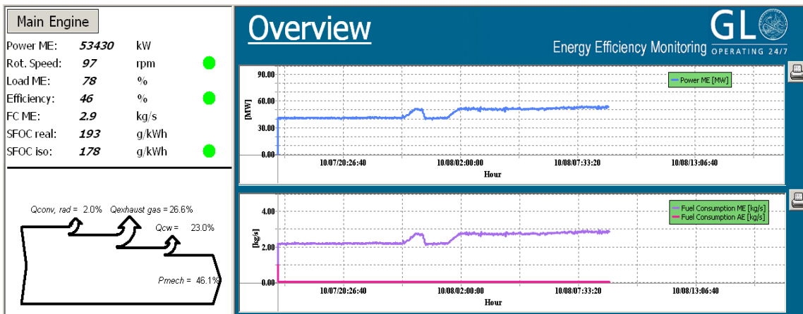
Fig.7: Energy Efficiency Monitoring for main engine
