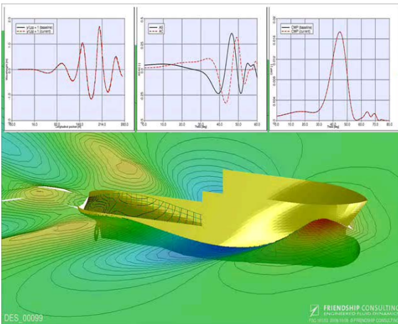
Fig.2: Hull lines optimization
